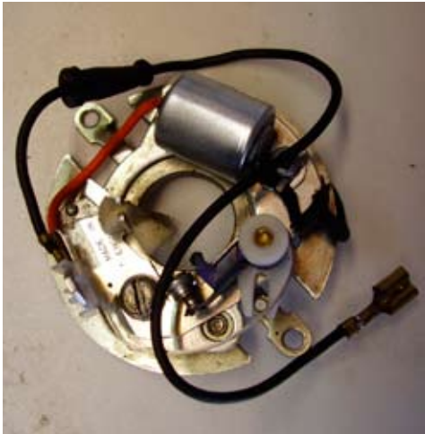
25D baseplate with points and condenser for roadside repair
