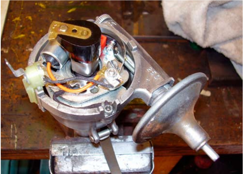
25D Dizzy with points and condenser
